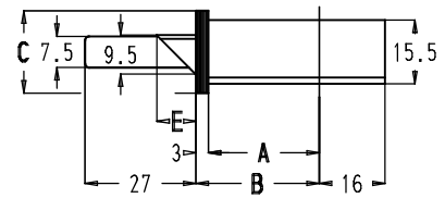
Flat faceplate
