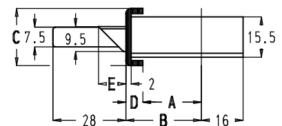
U-faceplate
